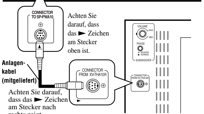
Aktiv-Sub-Woofer (SP-PWA10)
